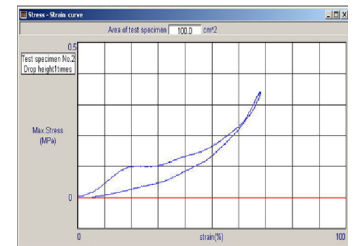
Stress-Strain curve
